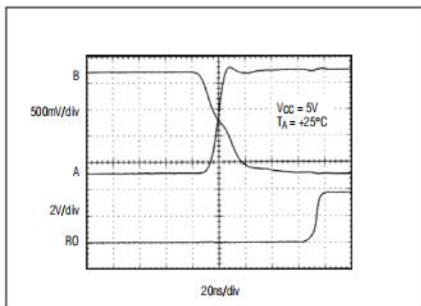
Figure 14. GM490E/GM491E Receiver t_{PLH}
