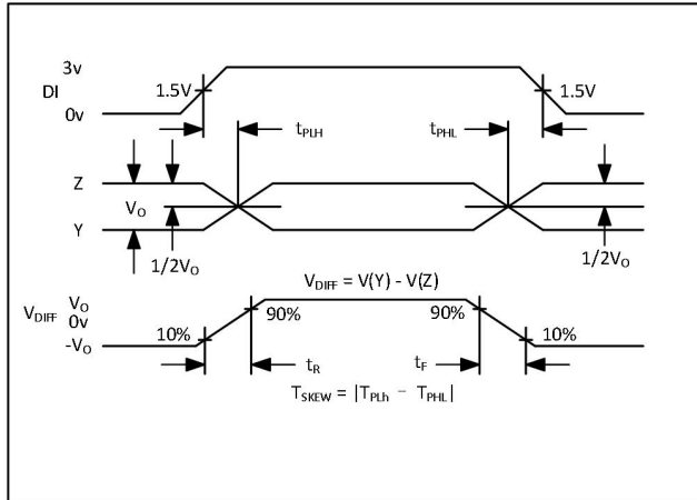
Figure 8. Driver Propagation Delays
